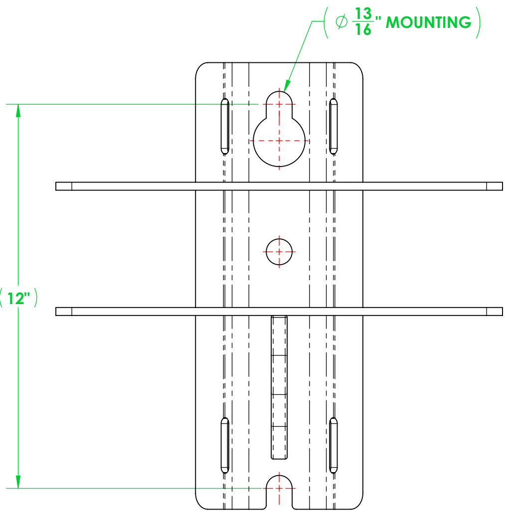
DETAIL A
